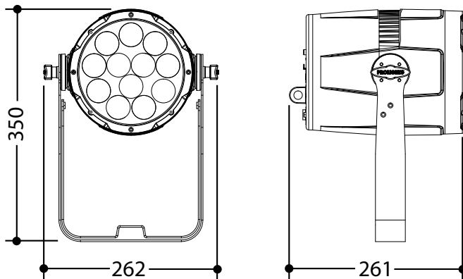
Technical drawing
