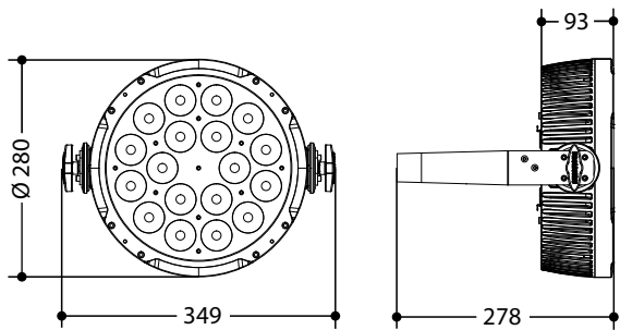
Technical drawing
