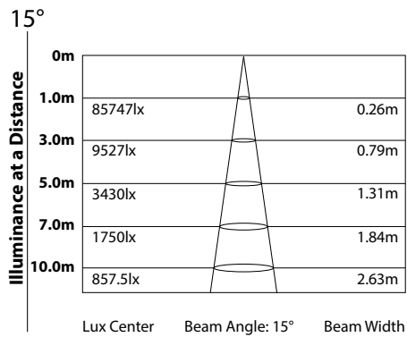
Photometric data
