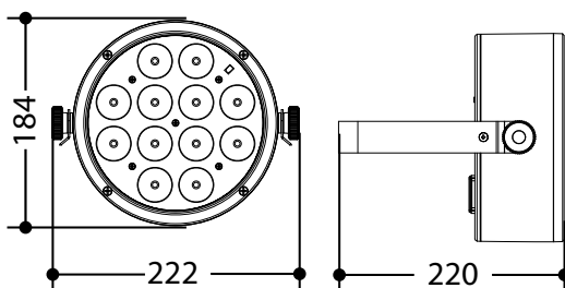
Technical drawing
