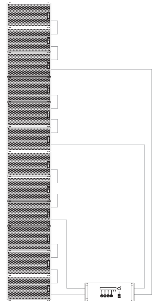
NXAMP4X4 powering 12 X GEO M12
