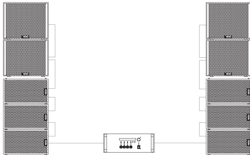
NXAMP4X4 powering 3 X GEO M12 and 2 X MSUB18 per side
