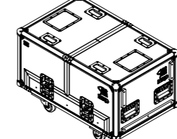
GMT-3CASE M10 Flight case for 3 x GEO M10, both side opening
